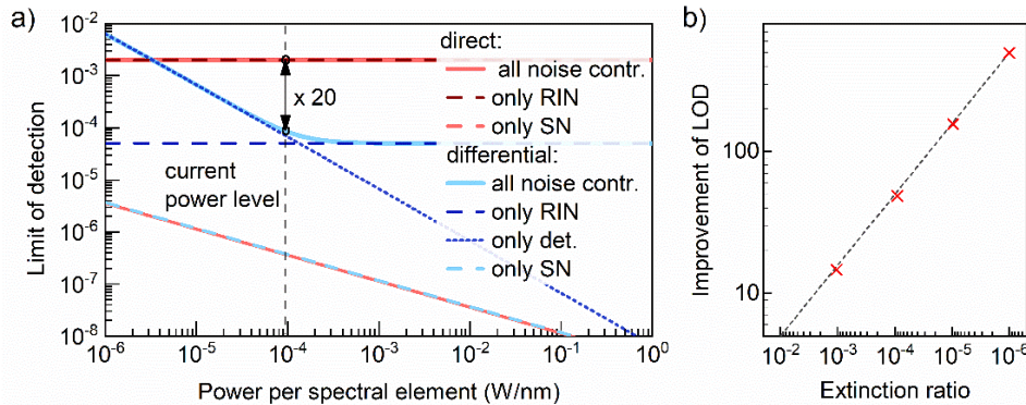
Fig. 4. (a) Calculated limit of detection for increasing power per spectral element in the direct and the differential configuration for an extinction ratio of 6 \times 10^{-4} and a constant relative intensity noise (RIN) of 0.2%. SN: shot noise. (b) Ratio of the direct and the differential LOD for four different extinction ratios in the intensity-noise-limited regime (red crosses) and 1/\sqrt{4\Delta} for comparison (dashed black line).
