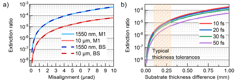
Fig. 2. (a) Simulated decrease of extinction ratio for misalignment of two different optical elements in the interferometer at 1550 nm and 10 \mu\text{m} central wavelength. (b) Simulated decrease of extinction ratio depending on the difference in substrate thickness of beam splitter and beam combiner for different input pulse durations. Shaded area: typical thickness tolerances specified by the manufacturer.
