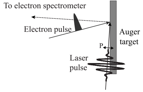
FIG. 1. Basic arrangement of electron pulse duration measurement. P indicates the direction of polarization of the laser pulse.
