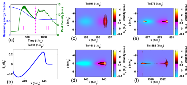
FIG. 6. Example of the simulated electron bunch evolution. The original bunch parameters are \sigma_r = 6.1 \mu\text{m} (corresponding to d \approx 6 mm), \sigma_z = 1.4 fs, n_p = 3.6 \times 10^{18} cm ^{-3} , and n_b/n_p = 0.31 . The density profile was a step function, starting at t = 47 . (a) Peak electron bunch density and REF vs time. After reaching quasistatic saturation [38] at t \sim 700 , the value of the peak density jumps between the main driver and secondary bunch ( \sim 4c/\omega_p behind main driver). (b) The magnitude profile of the longitudinal wakefield. (c)–(f) Bunch density and longitudinal electric field at different time steps.
