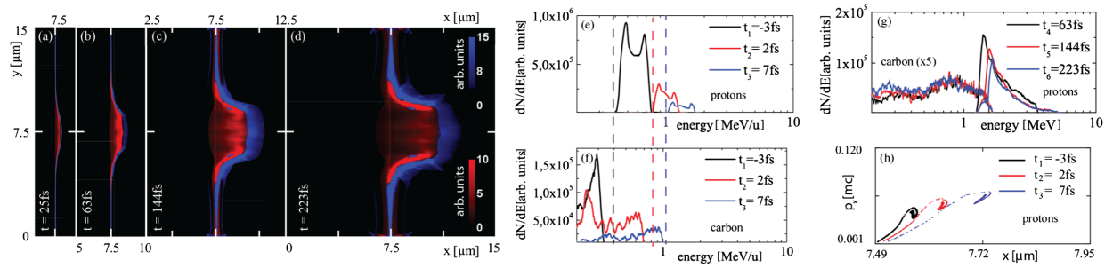
FIG. 3. Data from 2D-PIC simulation. (a)–(d) Spatial proton (blue) and carbon (red) ion density distribution in the x - y plane at different times (given in the figure caption) after the arrival of the peak of the Gaussian (in space and time) laser pulse. The spectral evolution during the laser-target interaction of protons (e), carbon ions (f), and after the interaction (g). In (h) the proton phase space during the interaction is revealing the characteristic spiral structure for RPA.
